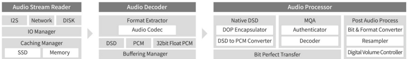
crtež 2 - ROSE audio server
